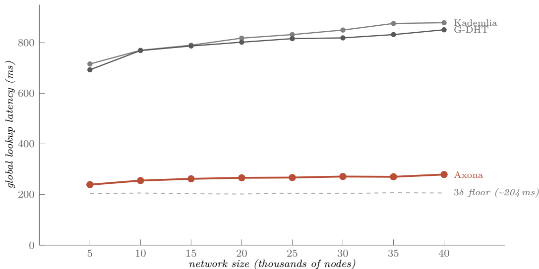
Figure 3: Global lookup latency versus network size at 5,000, 10,000, 15,000, 20,000, 25,000, 30,000, 35,000, and 40,000 nodes ( 8\times scaling), plotted against the Dabek 3\delta analytical floor (gray dashed). Kademia climbs from 716 to 879 ms as the log- N hop tax compounds; G-DHT tracks Kademia almost identically on global lookups (the geographic prefix only helps regional cells). Axona hugs the floor in a tight 239–279 ms band across the whole range ( 1.17\text{--}1.35\times the 3\delta floor) and is essentially flat from 15,000 nodes onward. All success rates 100%. Data: sim v0.93.0 / @axona/protocol v1.1.3, May 2026.
